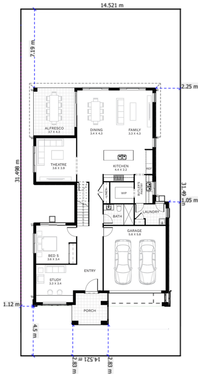
GROUND FLOOR
