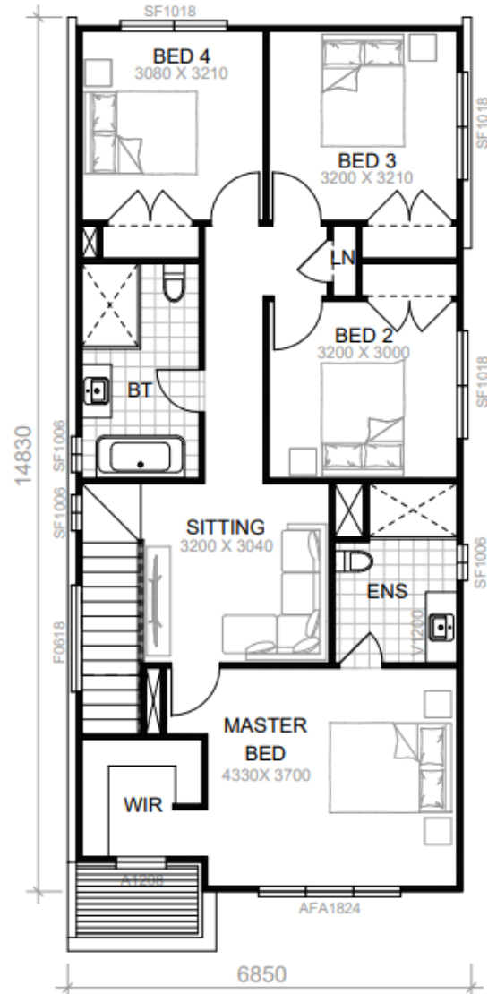
FIRST FLOOR
