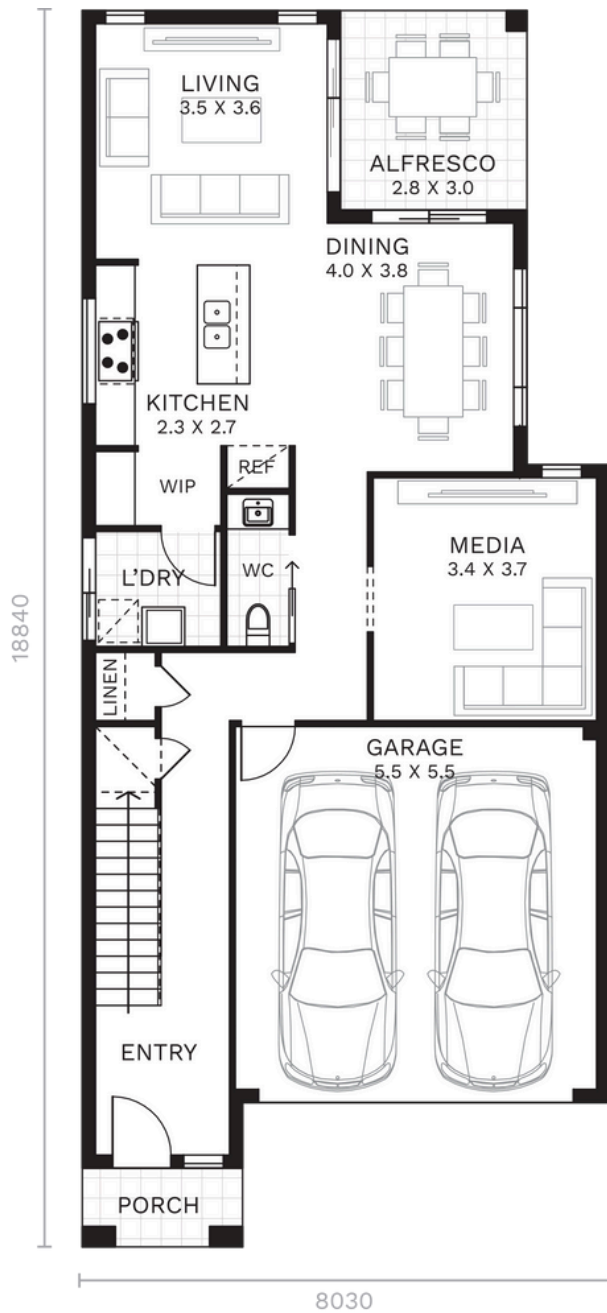
GROUND FLOOR
